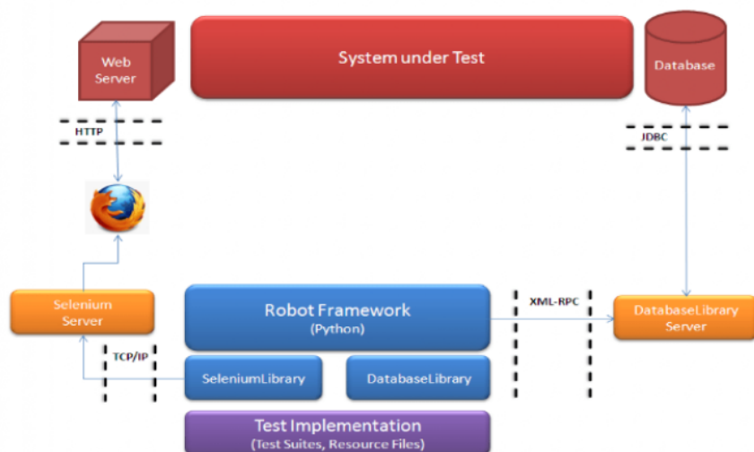
Figure 1: Main structure of Robot Framework.
