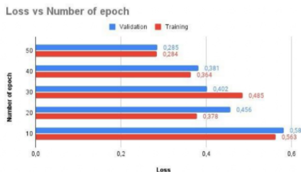
Figure 8: Training and Validation Losses
