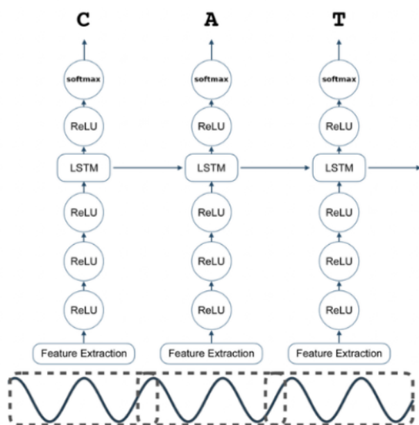
Figure 1: DeepSpeech architecture
