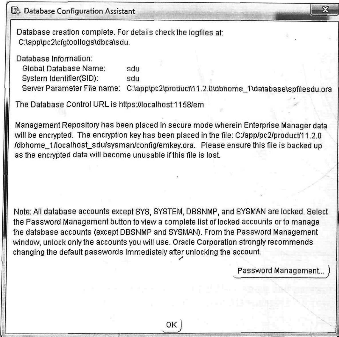
Figure 2.4.9. Database Configuration Assistant.
