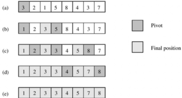
Figure 3. Quick sort example for sorting 8 elements in an array
