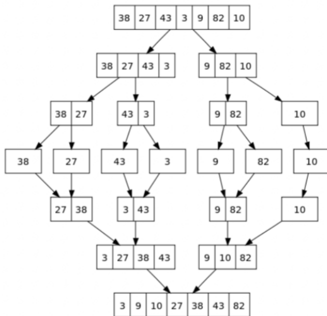
Figure 4. Merge sort example for sorting 7 elements in an array
